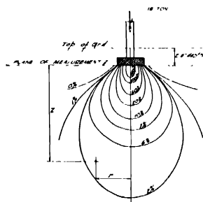
Pressure bulb for 16-ton load on 4-ft. by 4-ft. base.
